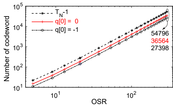
Fig. 4. The total number of codeword of the 1 st -order fully differential modulator with different initial feedback and OSR.
